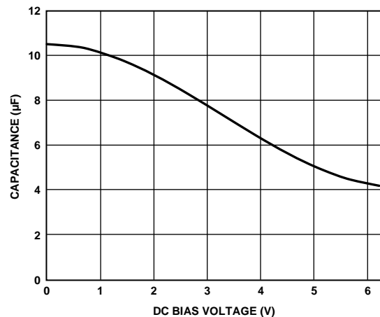
Figure 45. Typical Capacitor Performance
